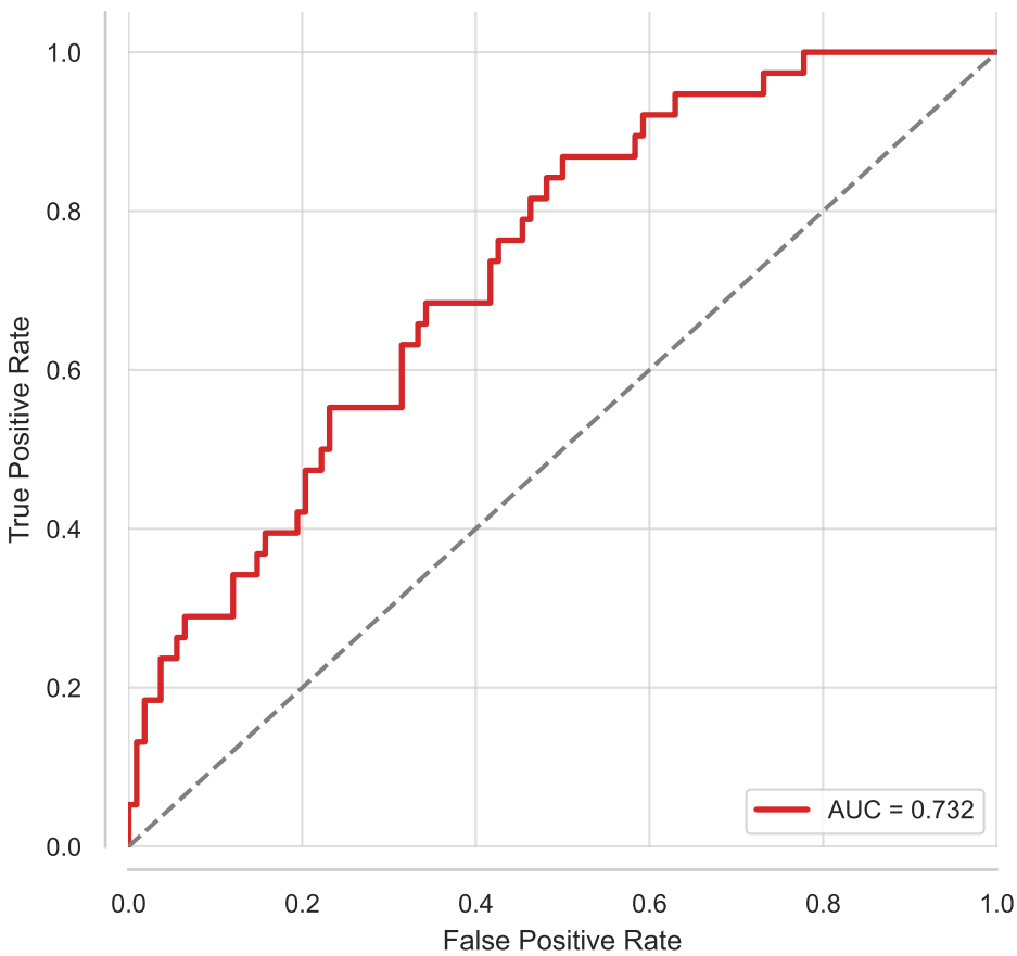
ROC Curve - HGB
